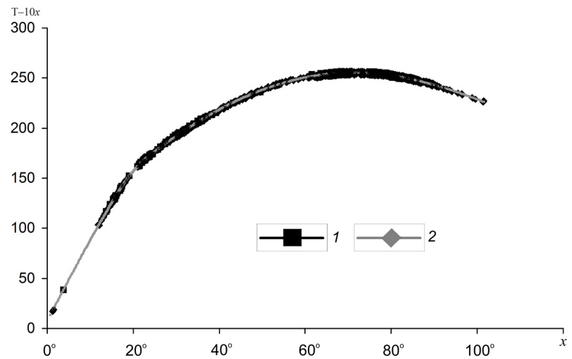
Fig. 3. Comparison of the experimental and theoretical travel-time curve (the number of points of locus – 12 971): 1 – experimental; 2 – theoretical
